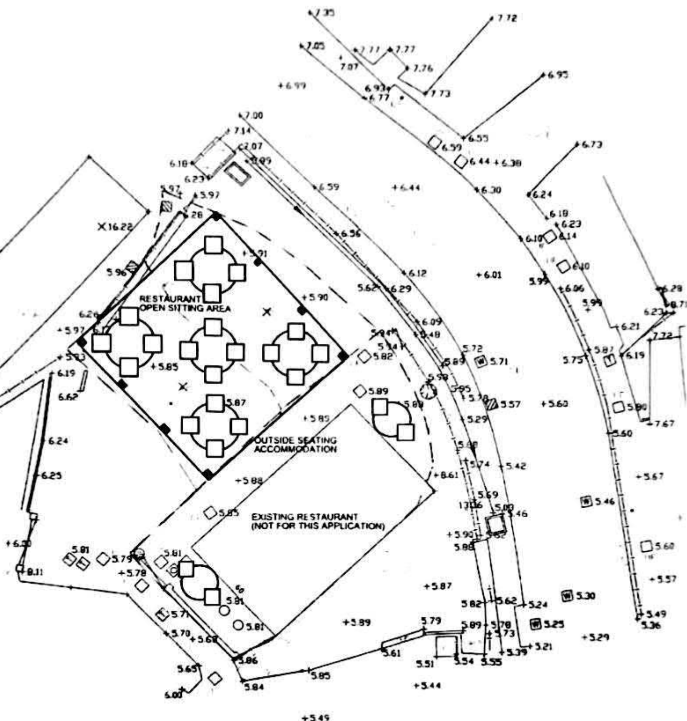
GROUND FLOOR SEATING LAYOUT PLAN (FOR INFORMATION ONLY)
